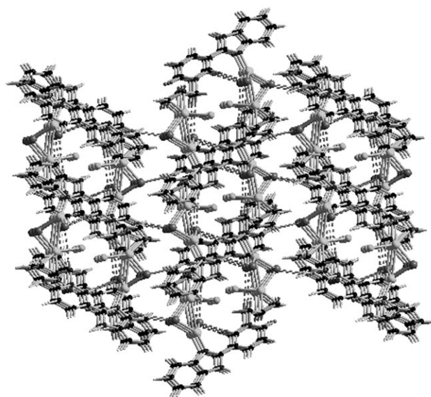
Figure 2. a) Crystal structure of 2 in which four Cu atoms and two L^2 ligands make up a 22-membered ring and all of the Cu atoms display distorted trigonal geometry. b) Packing view of 2 revealing a pseudo-three-dimensional polymer through weak supramolecular interactions along the c axis with a D\cdots Br distance (dotted lines) of 2.804 Å.
